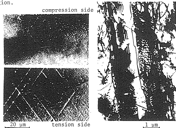
Fig.1 SEM micrographs of an etched (110) side surface of a [110] bent silicon crystal at 560°C.
