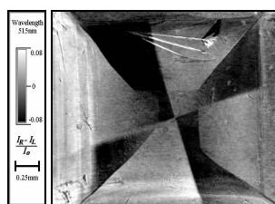
Figure 1. Circular Dichroism in 1-8-Dihydroxyanthraquinone.
