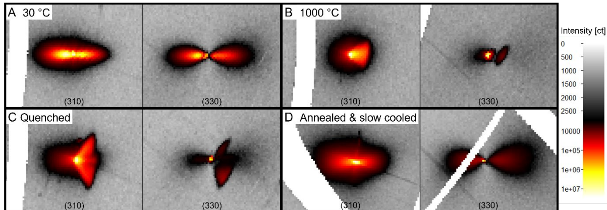
Figure 1. : Diffuse scattering in the hk0 -plane in Sanidine from the Vesuvio, Italy. A. Untreated crystal. B. In-situ at 1000 °C. C. Quenched to 30 °C. D. Different crystal from the same sample that was annealed at 1050 °C for one week and slowly cooled over 8 hours.
