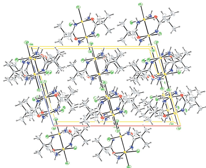
Figure 5 Crystal packing of [\text{Pt}_2\text{Cl}_4(\text{NH}_3)_2\{\mu\text{-HN}=\text{C}(\text{O})\text{Bu}'\}_2] , viewed along [010]. Ellipsoids drawn at the 30% probability level. Atom color coding: white for hydrogen, green for chlorine, blue for nitrogen, gray for carbon and red for oxygen.
