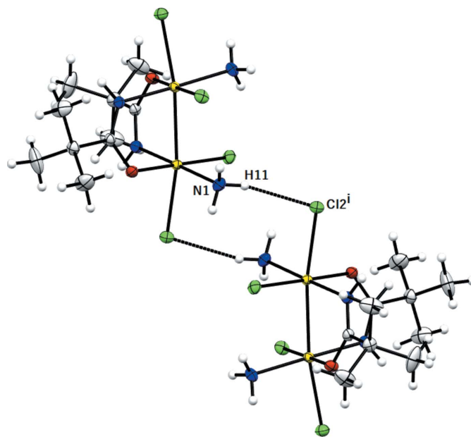
Figure 6 MERCURY drawing of two molecules of [\text{Pt}_2\text{Cl}_4(\text{NH}_3)_2\{\mu\text{-HN}=\text{C}(\text{O})\text{Bu}'\}_2] linked by an intermolecular hydrogen bond [N1...Cl2 i 3.406 (2) Å, (N1)H11...Cl2 i 2.54 Å, N1–H1...Cl2 i 166°; symmetry code: (i) 1 - x, -y, 1 - z ]. Ellipsoids drawn at the 30% probability level. Atom color coding: white for hydrogen, green for chlorine, blue for nitrogen, gray for carbon and red for oxygen.
