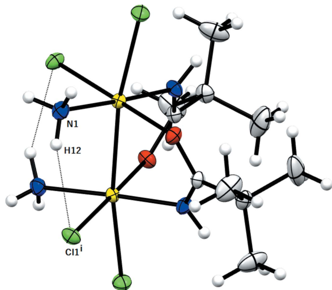
Figure 4 MERCURY drawing of [\text{Pt}_2\text{Cl}_4(\text{NH}_3)_2\{\mu\text{-HN}=\text{C}(\text{O})\text{Bu}'\}_2] showing the intramolecular hydrogen bond interaction [N1...Cl1 i 3.176 (3) Å, (N1)H12...Cl1 i 2.46 Å, N1–H12...Cl1 i 140°; symmetry code: (i) 1 - x, y, -z + \frac{1}{2} ]. Ellipsoids drawn at the 30% probability level. Atom color coding: white for hydrogen, green for chlorine, blue for nitrogen, gray for carbon and red for oxygen.
