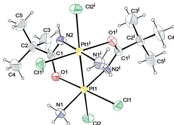
Figure 3 ORTEP drawing of the final structure model of the [Pt 2 Cl 4 (NH 3 ) 2 {μ-HN=C(O)Bu'} 2 ] complex. Symmetry code: (i) 1 − x , y , \frac{1}{2} − z . Ellipsoids drawn at the 30% probability level. Atom color coding: white for hydrogen, green for chlorine, blue for nitrogen, gray for carbon and red for oxygen.
