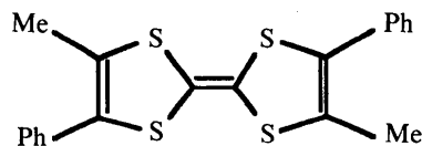
Fig. 1. Structure of DMDPh-TTF.
