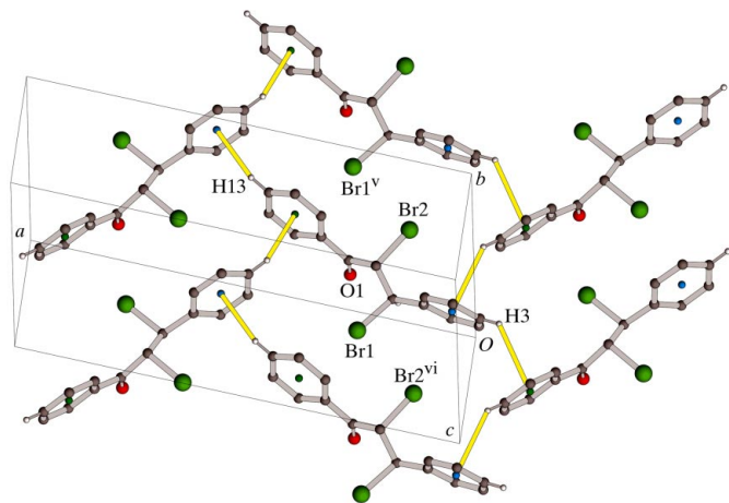
Figure 3 A detail of (I), showing how C—H \cdots\pi interactions involving atoms H3 and H13 provide coherence between herring-bone-like sheets of molecules. Note also how a Br atom is positioned approximately trans to every C—H \cdots\pi bond (see Comment ). H atoms not involved in the interactions shown have been omitted. [Symmetry codes: (v) x, y + 1, z ; (vi) x, y - 1, z .]
