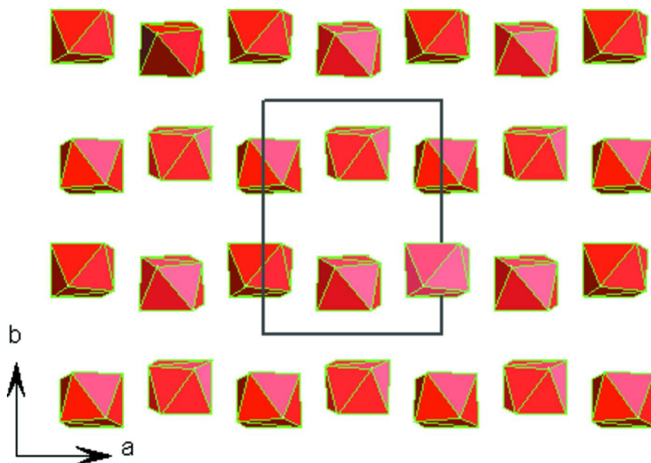
Figure 2 Projection of \text{EuO}_8 dodecahedra viewed along [0\ 0\ 1] direction.
