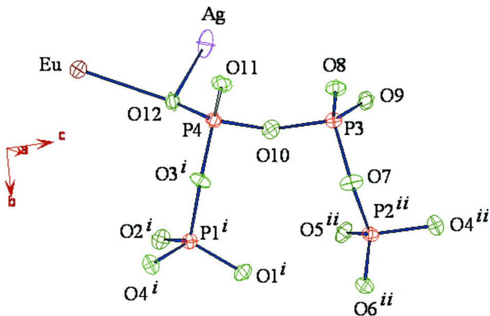
Figure 3 The sequence of \text{PO}_4 tetrahedra in \text{AgEu}(\text{PO}_3)_4 , with displacement ellipsoids drawn at the 50% probability level. [Symmetry codes: (i) 1-x, 2-y, 2-z ; (ii) 1-x/2, 2-y, 3-z ]
