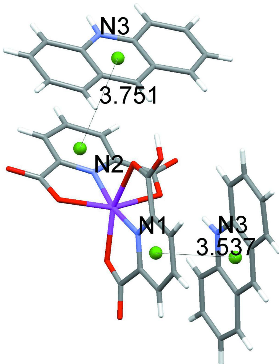
Figure 3 Representation of \pi - \pi stacking in (acrH)[Zn(pydcH)(pydc)] \cdot 5H_2O .
