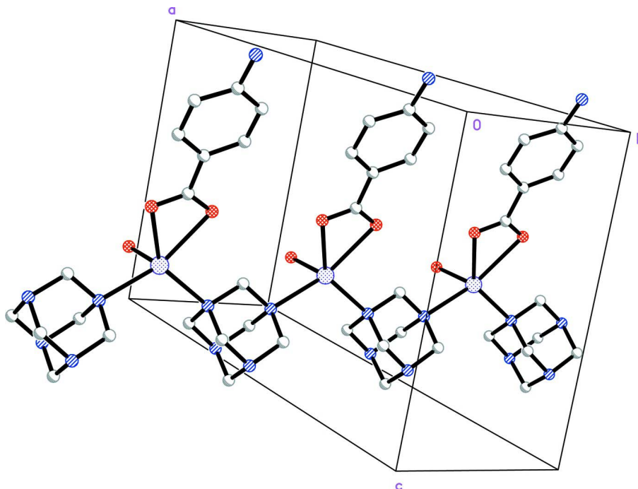
Figure 2 Part of the polymeric chain in the title compound.
