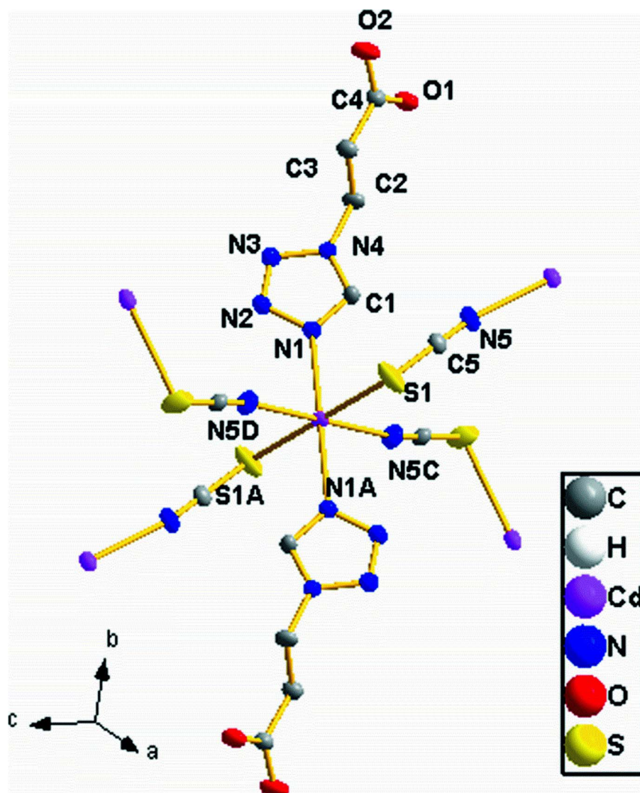
Figure 1 coordination environments of cadmium atoms in the title coordination polymer. Displacement ellipsoids are drawn at the 30% probability level. H atoms have been omitted for clarity.
