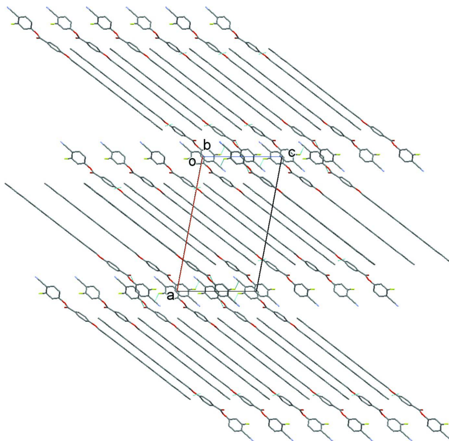
Figure 2 The packing arrangement of molecules viewed along the b axis. H atoms have been omitted for clarity
