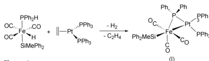
Figure 1 The reaction scheme for the synthesis of (I).
