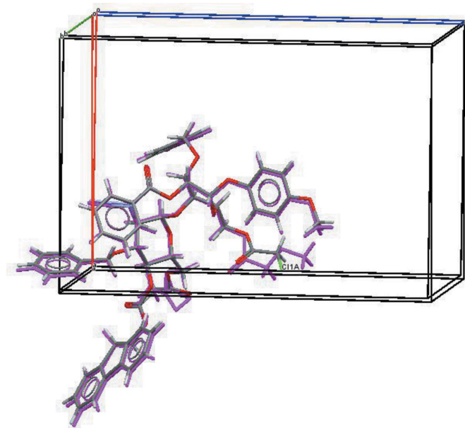
Figure 3 An overlap view ( Mercury ; Macrae et al. (2008) of the cell and asymmetric-unit atoms for the isostructural molecules (I) (atom colours) and (II) (in purple). The Cl atom in (I) is labelled to highlight the different pendant groups.
