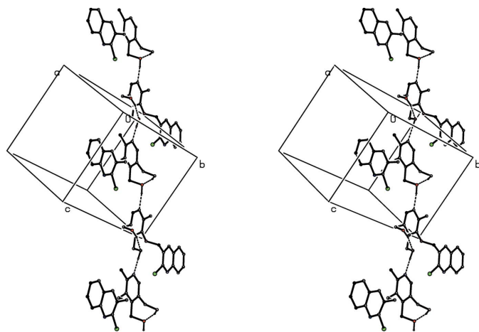
Figure 12 A stereoview of part of the crystal structure of compound (V) showing the formation of a C(7) chain formed by O-H \cdots N hydrogen bonds and running parallel to [10\bar{1}] . For the sake of clarity, H atoms bonded to C atoms have been omitted.
