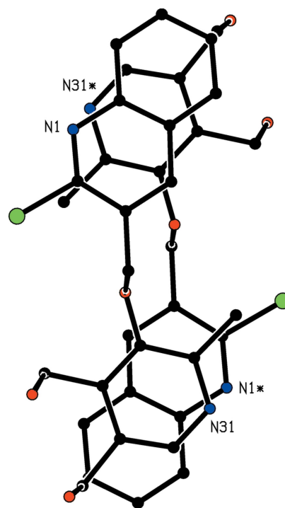
Figure 13 Part of the crystal structure of compound (V) showing the formation of a centrosymmetric \pi -stacked dimer. For the sake of clarity, H atoms have all been omitted. Atoms marked with an asterisk (*) are at the symmetry position (-x + 1, -y + 1, -z + 1) .
