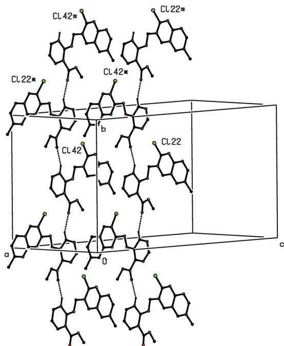
Figure 11 Part of the crystal structure of compound (III) showing the formation of a chain running parallel to the [010] direction and containing alternating molecules of types 2 and 4. For the sake of clarity, H atoms not involved in the motifs shown have been omitted. Atoms marked with an asterisk (*) or a hash (#) are at the symmetry positions (-x + 1, y + \frac{1}{2}, -z + \frac{1}{2}) and (x, y + 1, z) , respectively.
