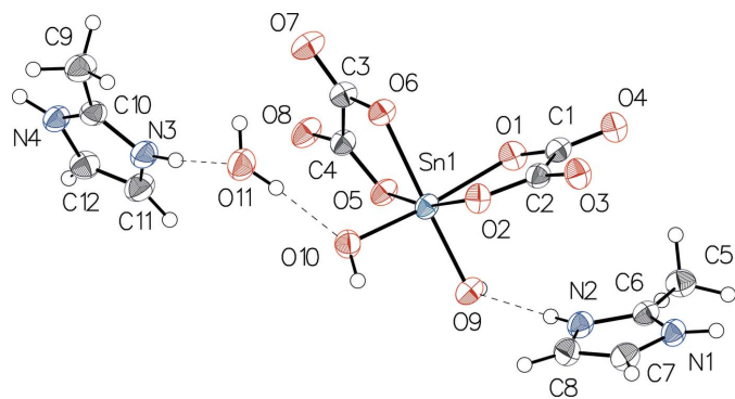
Figure 1 The structure of the molecular components in the title compound, with displacement ellipsoids drawn at the 50% probability level. H atoms are drawn as spheres of arbitrary radius and hydrogen bonds are shown as dashed lines.
