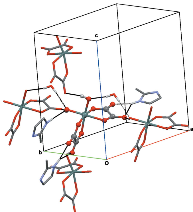
Figure 2 A view of a central stannate dianion (ball-and-stick representation) surrounded by its hydrogen-bonded neighbours (stick representation), viz three cations, two water molecules and four other stannate anions. Hydrogen bonds are displayed as black dotted lines and H atoms not involved in hydrogen bonding have been omitted for clarity.
