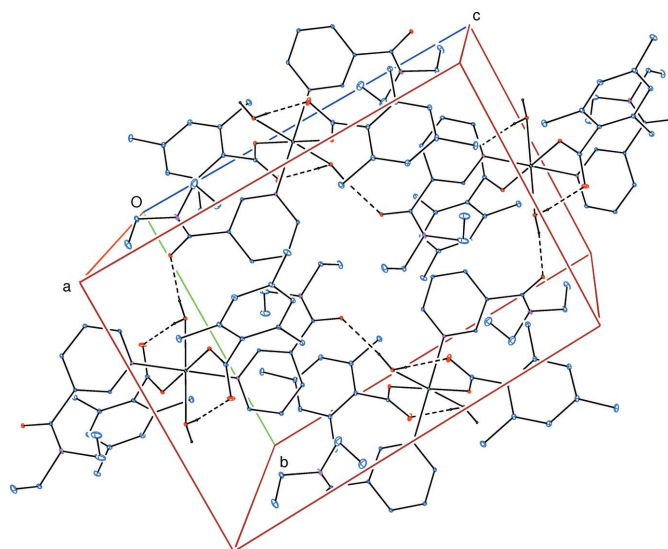
Figure 2 Part of the crystal structure viewed approximately down [100]. Intra- and intermolecular O—H...O hydrogen bonds, shown as dashed lines, enclose R_4^4(32) ring motifs. Only one part of the disordered group and only H atoms involved in hydrogen bonding have been included for clarity.
