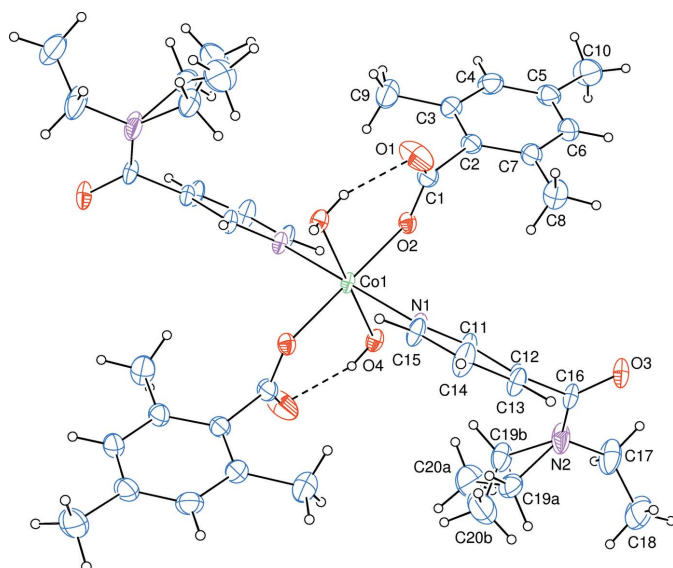
Figure 1 The molecular structure of the title complex with the atom-numbering scheme for the asymmetric unit. Unlabelled atoms are generated by symmetry code (1 - x , 1 - y , - z ). Displacement ellipsoids are drawn at the 40% probability level. Intramolecular O—H...O hydrogen bonds are shown as dashed lines.
