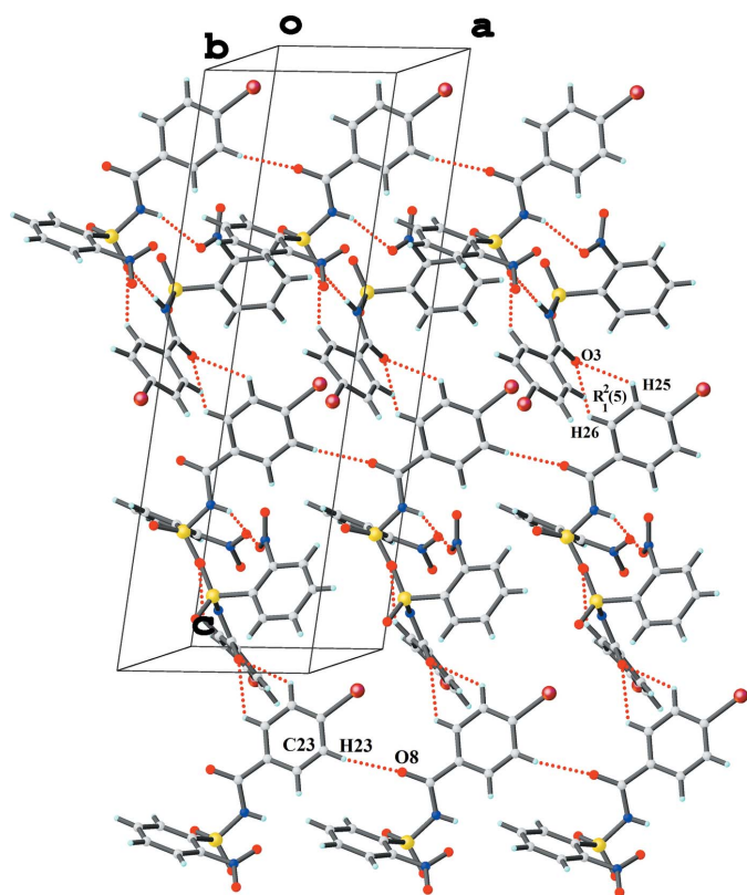
Figure 3 The crystal packing of (I), displaying the hetero R_2^2(11) dimeric supramolecular synthon. Molecules assemble along the a axis forming C (6) chains via C-H\cdots O interactions while two further C-H\cdots O interactions involving the same acceptor atom lead to the formation of an R_1^2(5) network.
