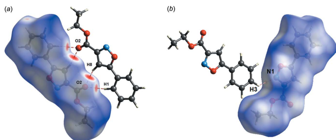
Figure 5 Hirshfeld surface mapped over (a) d_{\text{norm}} highlighting the regions of \text{C}-\text{H}\cdots\text{O} hydrogen bonding and (b) d_{\text{norm}} highlighting the region of \text{C}-\text{H}\cdots\text{N} hydrogen bonding.
