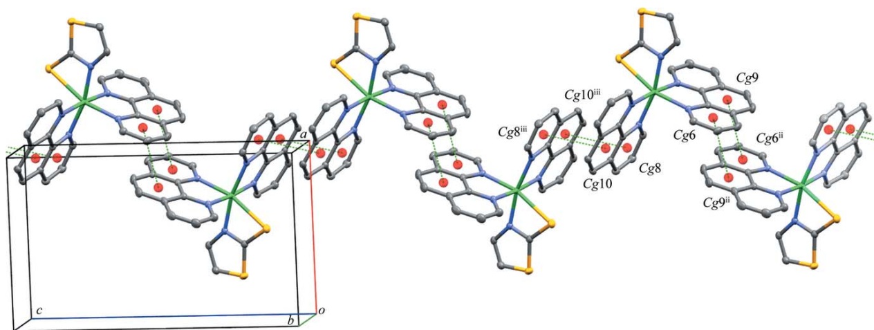
Figure 2 The arrangement of the complex cations in the crystal structure, forming zigzag \pi – \pi stacked chains extending parallel to the c axis. Green dashed lines represent \pi – \pi stacking interactions, red spheres represent centroids of the phenyl/pyridyl rings. \text{Cg}6 , \text{Cg}9 , \text{Cg}8 and \text{Cg}10 are the centroids of the N3/C14/C10–13, C7–C10/C14/C15, N5/C26/C22–C25 and C19–C22/C26/C27 rings, respectively. [Symmetry codes: (ii) 2 - x, 1 - y, 1 - z ; (iii) 2 - x, 1 - y, -z .]
