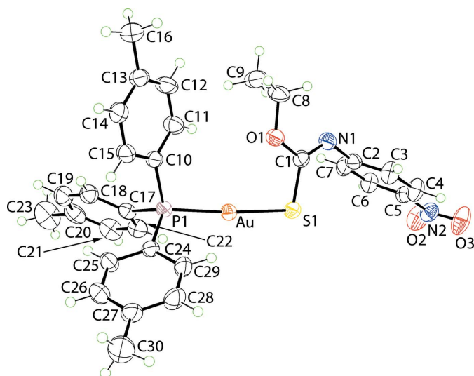
Figure 1 The molecular structure of (I) showing the atom-labelling scheme and displacement ellipsoids at the 50% probability level.
