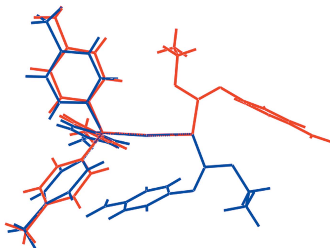
Figure 2 Overlay diagram of the molecular structures found in (I) ( P2 1 / c , red image) and (II) ( Cc , blue) forms of (4-tol) 3 PAu[SC(OEt)=NC 6 H 4 NO 2 -4]. The molecules have been overlapped so that the P–Au–S fragments are coincident.
