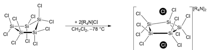
Figure 4 Synthesis of [R_4N]_2[Si_5Cl_{12}] ( R = nBu or Et).
