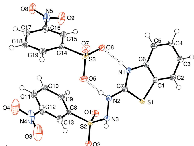
Figure 3 The asymmetric unit of (III) showing 50% displacement ellipsoids. Hydrogen bonds are indicated by double-dashed lines.
