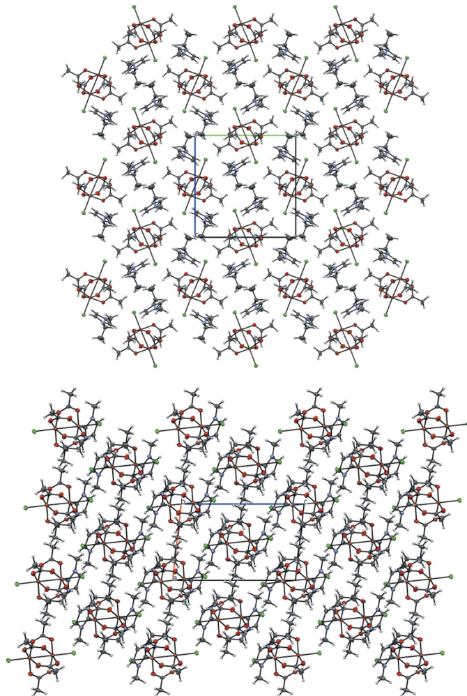
Figure 5 The packing of compound 1 , viewed along the a and b axes.
