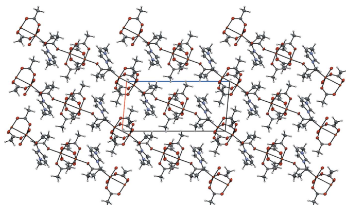
Figure 7 The packing of compound 3 , viewed along the b axis.
