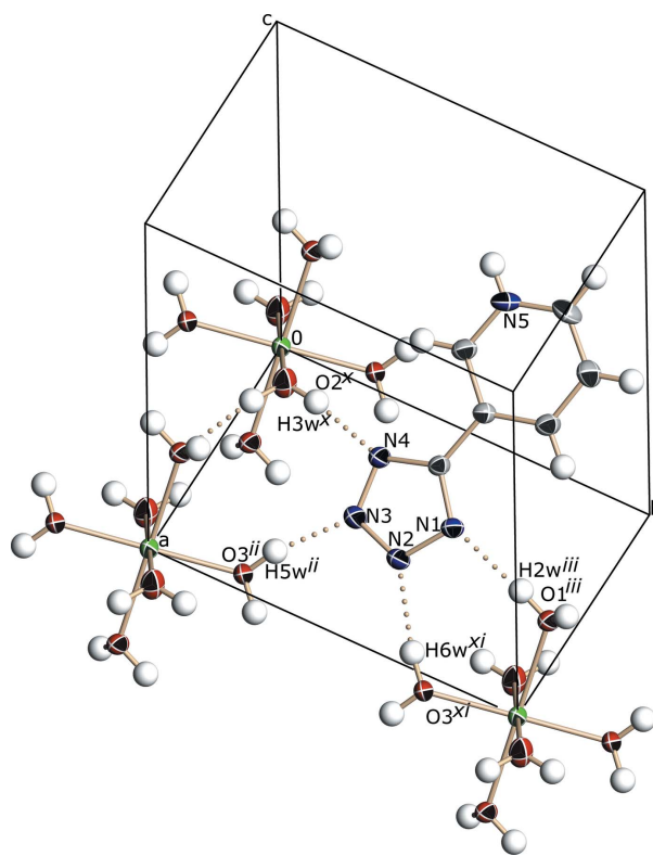
Figure 2 Partial crystal packing of the title compound, showing the hydrogen-bonding interactions between [Zn(H 2 O) 6 ] 2+ and the tetrazolidide ring. [Symmetry codes: (ii) -x + 1, -y + 1, -z + 1 ; (iii) -x + 1, -y + 2, -z + 1 ; (x) x, y - 1, z - 1 ; (xi) x + 1, y, z - 1 .]
