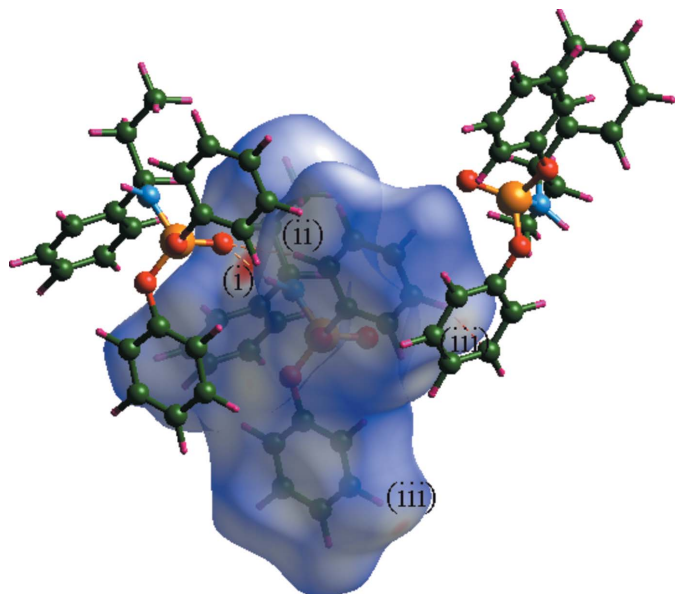
Figure 7 Hirshfeld surface map generated for the structure I . Two molecules are shown outside the surface to represent the N–H···O [label (i)], C–H···O [label (ii)] and typical C–H··· \pi [label (iii)] interactions with the molecule within the surface.
