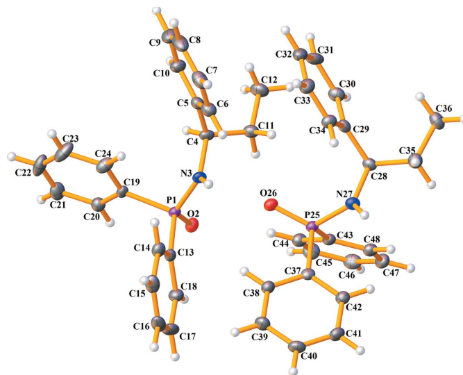
Figure 2 Displacement ellipsoid plot (50% probability) of the asymmetric unit of II , showing the atom-numbering scheme for non-hydrogen atoms. Hydrogen atoms are drawn as spheres of arbitrary radii.
