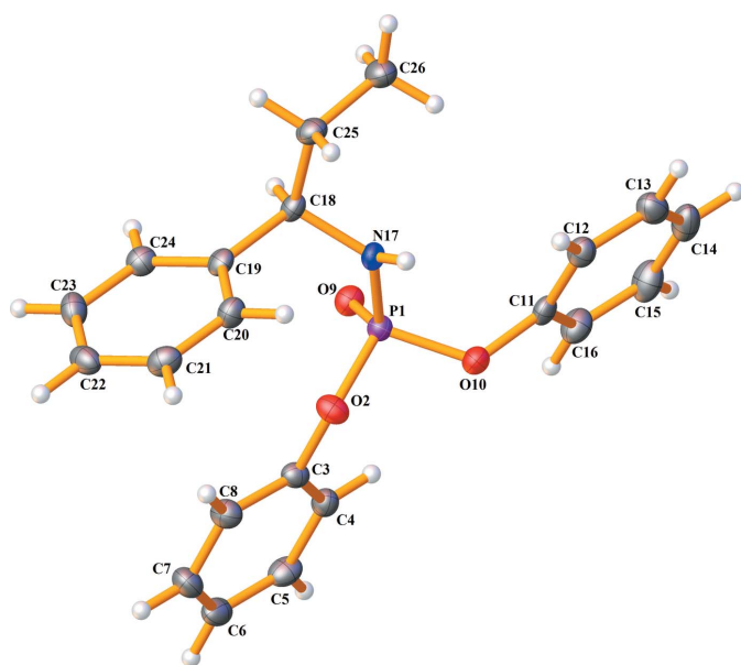
Figure 1 The asymmetric unit of I , showing the atom-numbering scheme for non-hydrogen atoms and displacement ellipsoids at 50% probability level. Hydrogen atoms are drawn as spheres of arbitrary radii.
