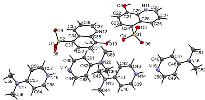
Figure 1 The molecular structure of the title compound with atom labeling. Displacement ellipsoids are drawn at the 50% probability level. H atoms are represented by spheres of arbitrary radius.
