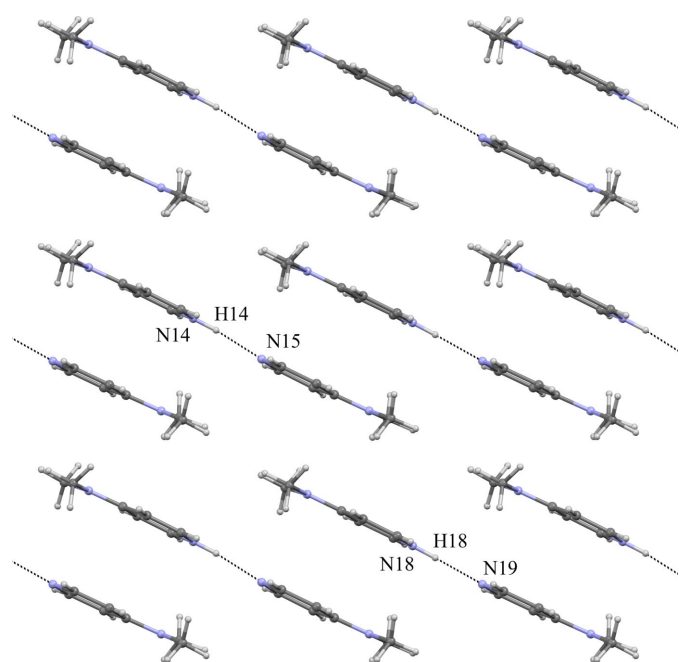
Figure 2 The layer structure of the [HDMAP·DMAP] + cationic unit in the ab plane. The intermolecular N—H···N hydrogen bonds are shown as dashed lines.
