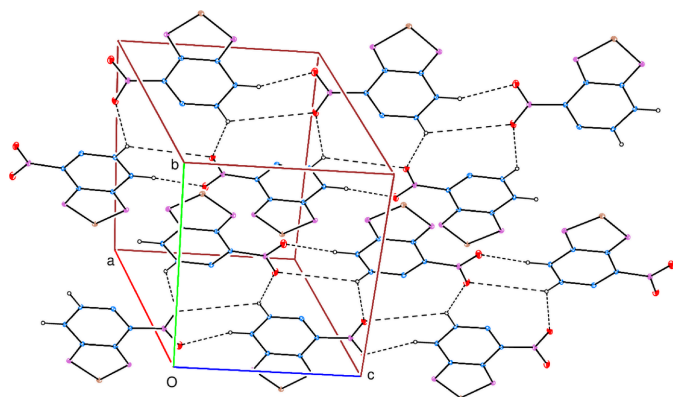
Figure 2 A partial packing diagram. Intermolecular C–H···O hydrogen bonds are shown by dashed lines.
