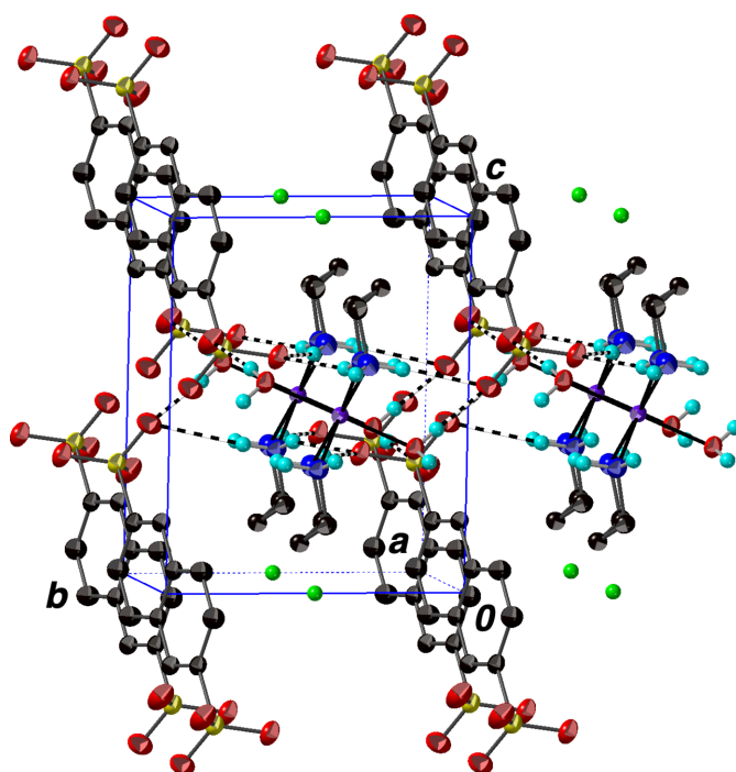
Figure 8 View of the packing in (II) showing the centroids (small green spheres) of cavities of radius ca. 2.5 Å in the anion layers.
