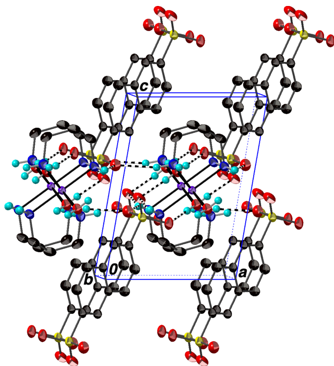
Figure 6 Packing diagram of (II) with the outline of the unit cell. The alternating layers of nickel complex cations and 2,6-nds anions are evident. O—H...O and N—H...O hydrogen bonds are shown as striped cylinders.
