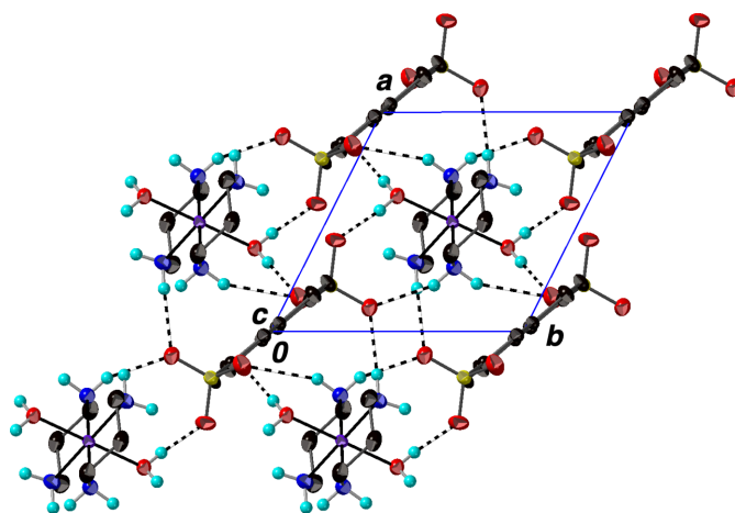
Figure 7 View of (II) perpendicular to the layers in the ab plane showing the alternating columns of cations and anions linked by the network of O—H...O and N—H...O hydrogen bonds (striped cylinders).
