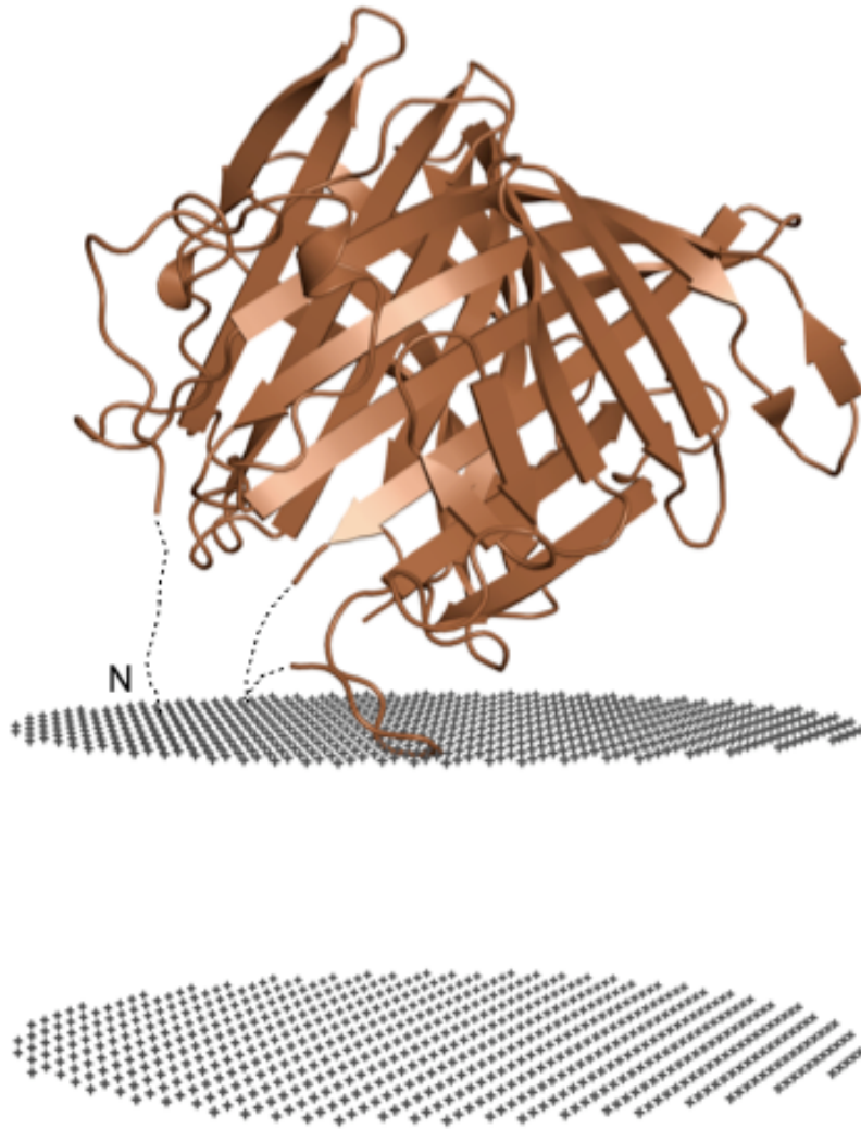
Figure S1. Model of NE1406 interacting with a membrane. The hydrocarbon boundary planes of the lipid bilayer (head groups of lipids go \sim 10 Å beyond these boundaries) are depicted as hashed disks. Dashed lines indicate the regions not modeled in the protein structure. The predicted N-terminus is indicated.
