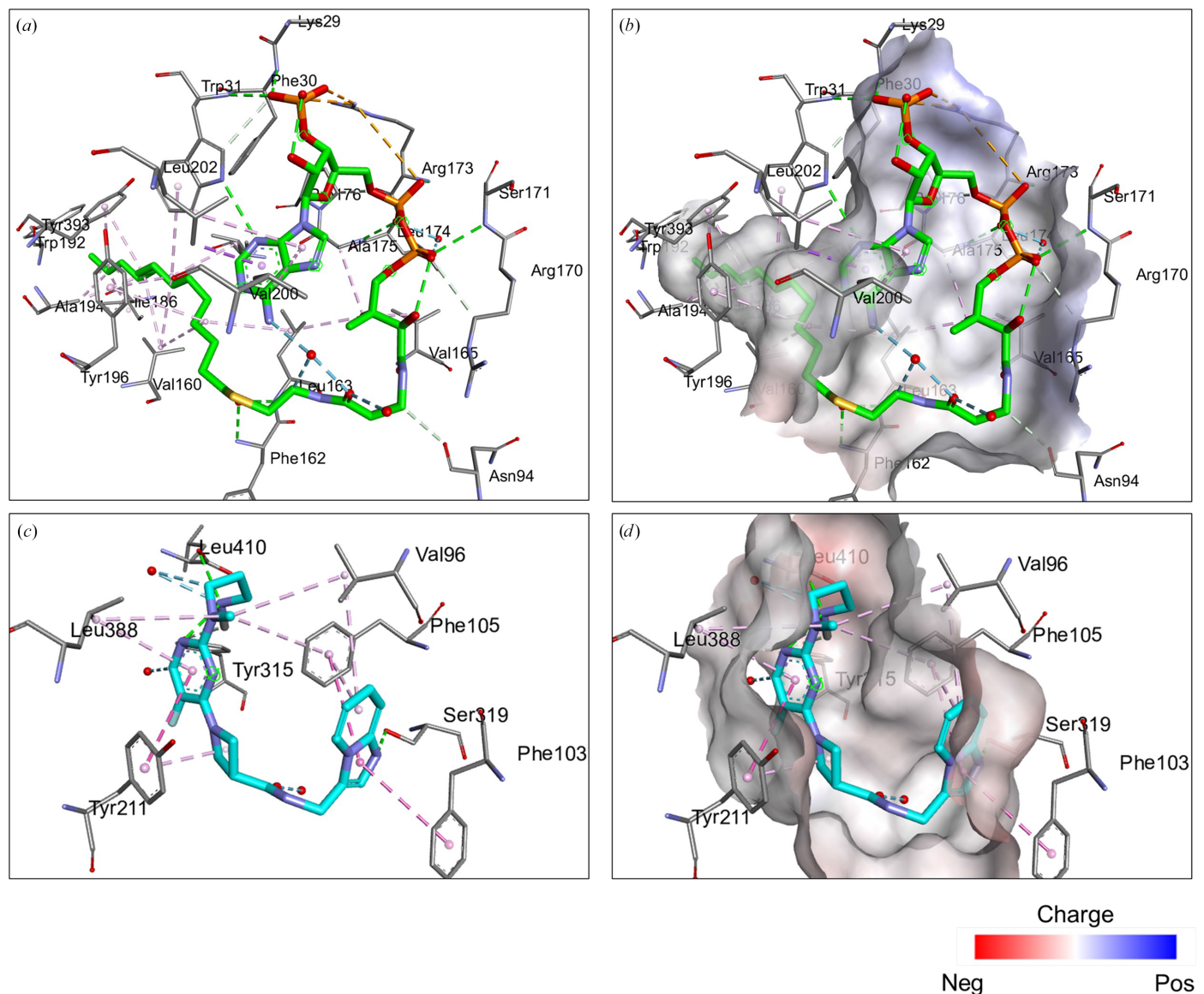
Figure 2 Myr-CoA and inhibitor (IMP-0001173) binding by Pv NMT. The interactions were analyzed with Discovery Studio Visualizer ( https://discover.3ds.com/discovery-studio-visualizer ). (a) Stick representation of amino-acid residues (gray) interacting with Myr-CoA (green). (b) The Myr-CoA-binding pocket is slightly positively charged [shown in the same view as in (a)]. (c) The inhibitor IMP-0001173 (shown in cyan) interacts with amino acids (gray). (d) IMP-0001173 has primarily electrostatic interactions in the peptide-binding pocket.
