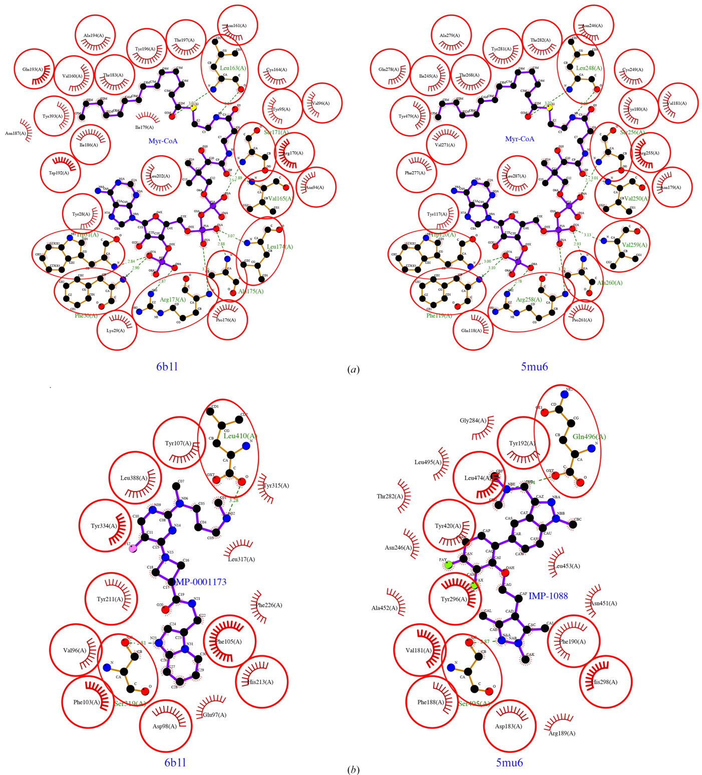
Figure 4 LIGPLOT -generated interaction plots for PvNMT (PDB entry 6b11) and HsNMT1 (PDB entry 5mu6) reveal (a) conserved Myr-CoA cavities and (b) differences in the peptide-binding cavity. The HsNMT1 structure (PDB entry 5mu6) has IMP-1088 within the peptide-binding pocket compared with IMP-0001173 in the PvNMT structure (PDB entry 6b11).
