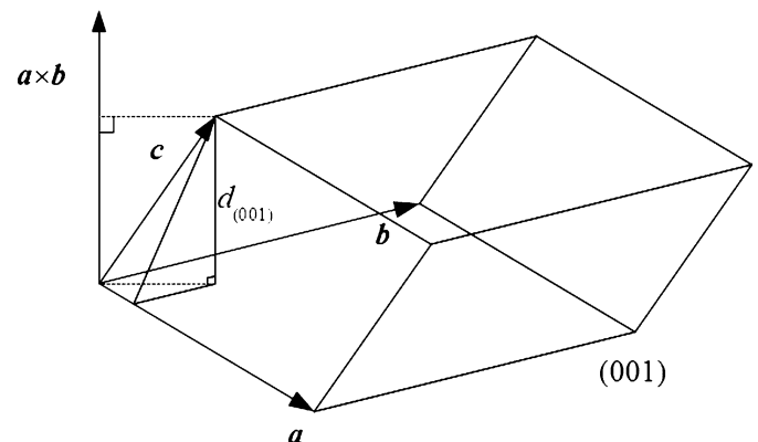
Figure 1 The interplanar distance of the (001) family.
