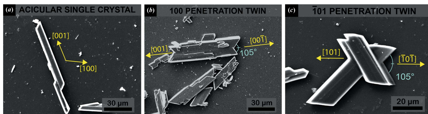
Figure 2 Gypsum crystals precipitated from G1 solution. (a) Acicular gypsum single crystals. (b) 100 penetration twin. (c) \bar{1}01 penetration twin.
