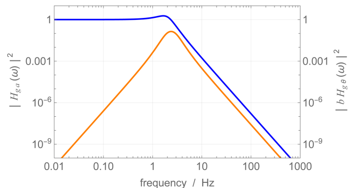
Figure 8 Mass-spring isolation system having \omega_m = 2 \times 2\pi Hz linear resonance frequency and \zeta_m = 0.4 damping ratio. Blue: squared transmissivity of the ground acceleration. Orange: squared transmissivity of the ground acceleration to the mass angular acceleration. The angular resonance frequency is \omega_\alpha = \sqrt{2}\omega_m . The radius of gyration is \sqrt{2}b/4 , where b is the spring separation.
