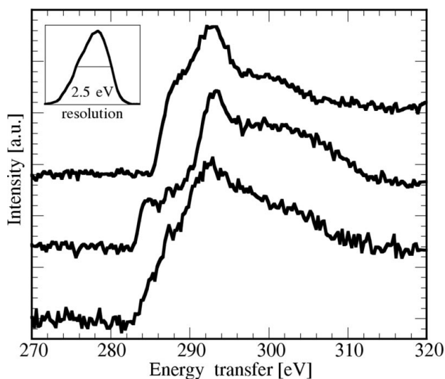
Figure 6 X-ray Raman spectra of (top to bottom): paraffin, coronene and asphaltene. Inset: measured energy resolution of the elastic peak, resulting from convolution of the incident-beam resolution and the analyzer resolution.
