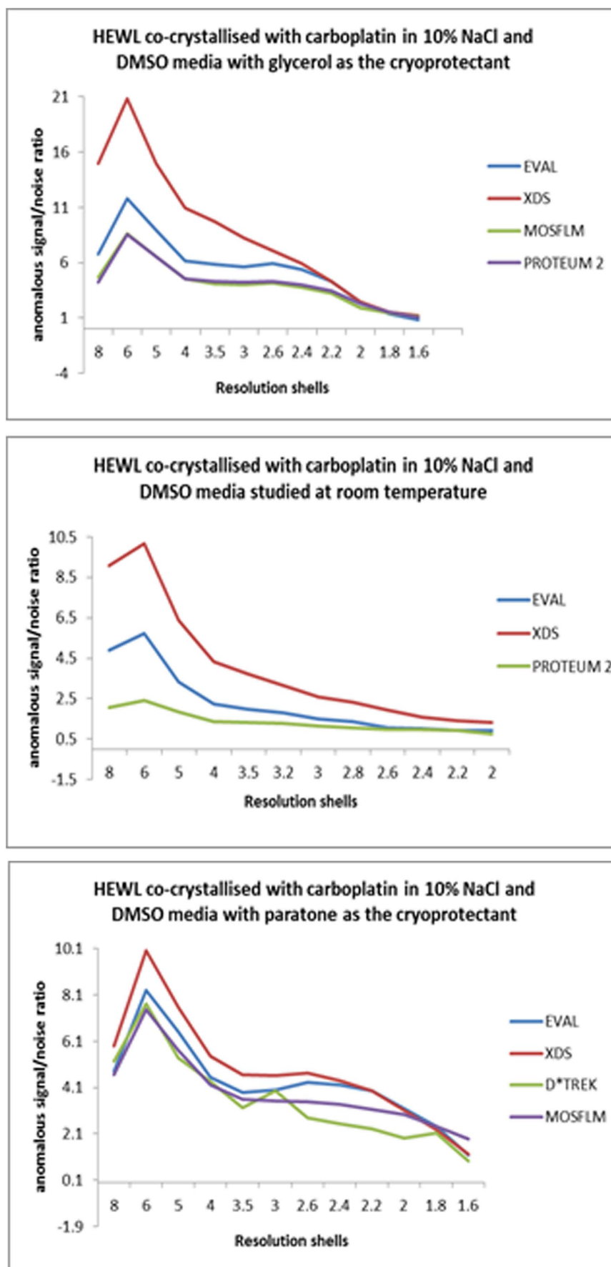
Figure S1 Anomalous signal to noise ratio for each crystal processed with the different software packages.
