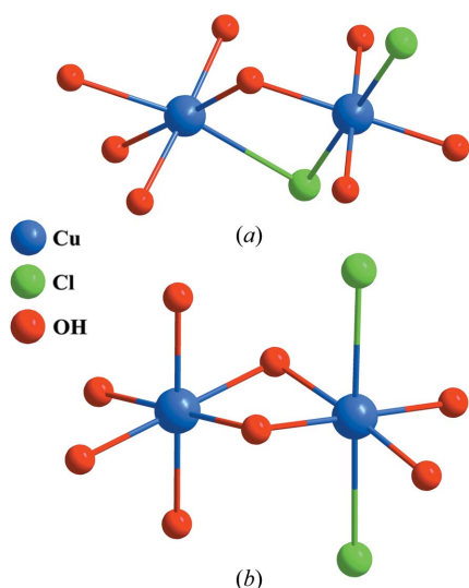
Figure 8 Possible octahedral Cu sites in two \text{Cu}_2(\text{OH})_3\text{Cl} polymorphs: (a) atacamite and (b) paratacamite.
