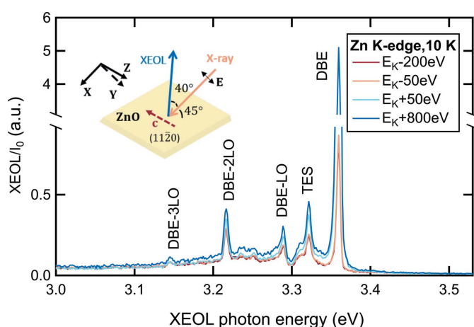
Figure 3 Normalized XEOL spectra measured at several selected X-ray energies across the Zn K-edge ( E_K = 9659 eV) at 10 K on a single-crystalline ZnO-(1120) wafer. The inset schematically illustrates the sample orientation relative to the polarization vector \mathbf{E} of the incident X-ray beam and the direction of the collected XEOL signal. Note that the measurement geometry corresponds to \mathbf{E} \perp \mathbf{c} (perpendicular) polarization mode. The emission bands are labeled based on PL studies (von Wenckstern et al. , 2007a,b; Wagner et al. , 2011), with the definition of the abbreviations given in Section 3.3.
