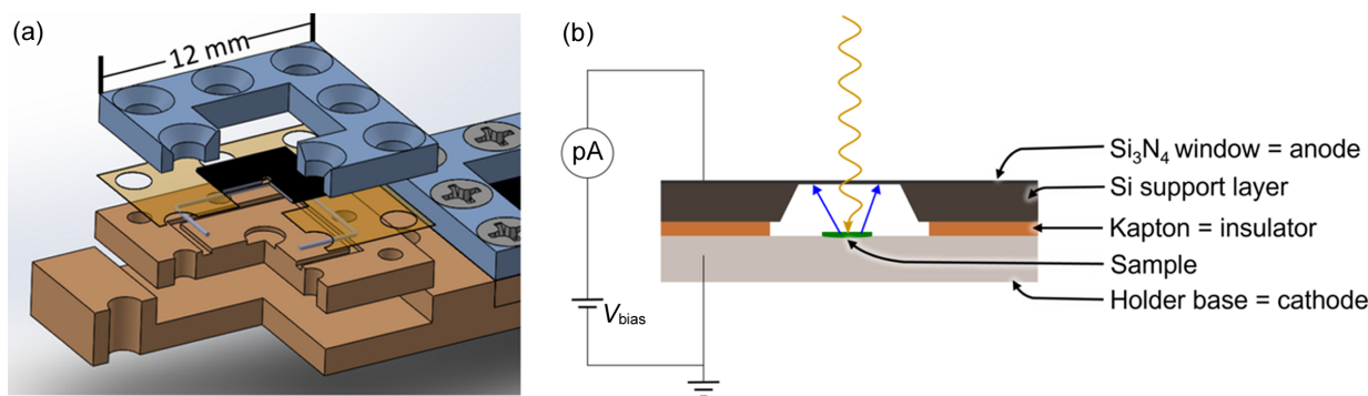
Figure 1 (a) Diagram of the holder including the holder base (brown), Kapton gasket (transparent orange), Si 3 N 4 membrane and Si frame (black), fiberglass (blue), and indium wire (gray). The distance between the sample and the window is less than 0.5 mm (Si support: 200 μm; Kapton gasket: 100 μm; sample well: 100 μm). (b) Side-view schematic of the holder with connections and incoming X-rays (yellow arrow) as well as ejected electrons from the sample (blue arrow) during measurements.
