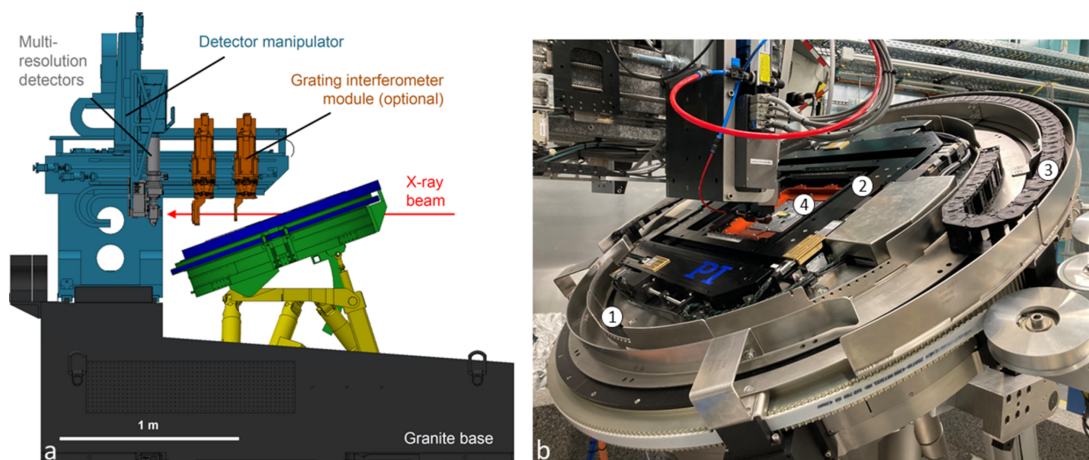
Figure 9 (a) Schematic side view of the LAMINO-II station highlighting the positioning modules for sample, detector and optical elements. (b) Photograph of the sample manipulator comprising a large air-bearing rotation axis (1) with open aperture in its centre, an x - y cross-table (2), as well as a cable drag (3) and a sample altogether tilted to an angle typical for laminographic measurements of a sample (4).
