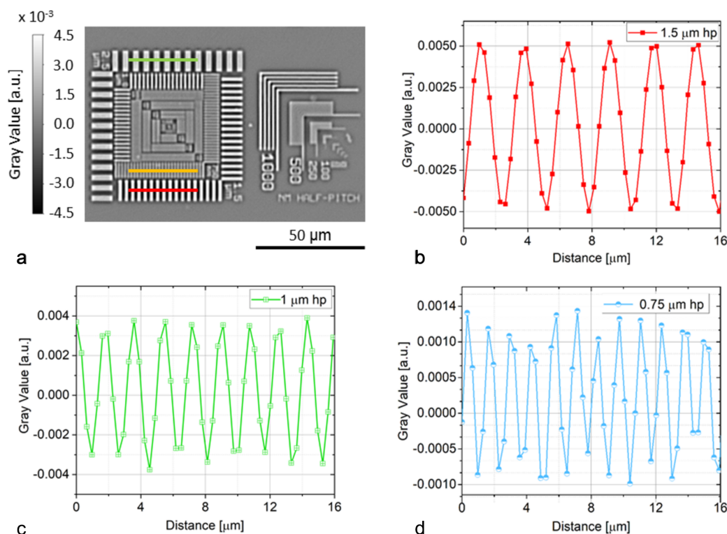
Figure 10 (a) Lateral slice through a 3D laminographic reconstruction (0.36 μm effective pixel size) of a resolution test pattern (model ANT HXRCA 25 nm, Edmonton, Canada), measured by LAMINO-II at IMAGE with a 45° tilt angle and with filtered whitebeam ( B = 1.8 T, 3 mm PG and 3 mm SiC filters, 3000 projections for a total measurement time of 10 minutes). The sample-to-detector distance of \sim 40 mm in combination with sufficiently closed primary slits of the beamline leads to features typical for beam propagation in the edge-enhancement regime (Cloetens et al. , 2001). (b)–(d) Grey value line profiles along the respective 1.5 μm, 1 μm, and 0.75 μm half pitch pattern. While from 1.5 μm to 1 μm the contrast decreases only slightly, it is strongly reduced for 0.75 μm, from which we estimate the achieved 3D spatial resolution to 1–2 μm.
