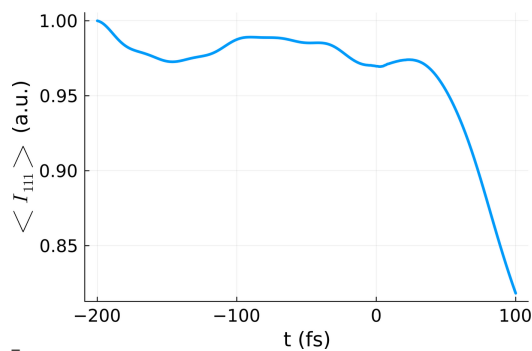
Figure 5 Volume-integrated 111 Bragg reflection intensity \langle I_{111} \rangle_{\text{vol,real}} . The integration was performed using the XTANT results for the doses marked in blue in Fig. 1. The calculation was performed for a silicon sample with 64 atoms in the simulation box, assuming a pulse duration of 6 fs FWHM and photon energy of 50 eV. The decay in the intensity observed after time zero reflects the progressing displacement of atoms.
