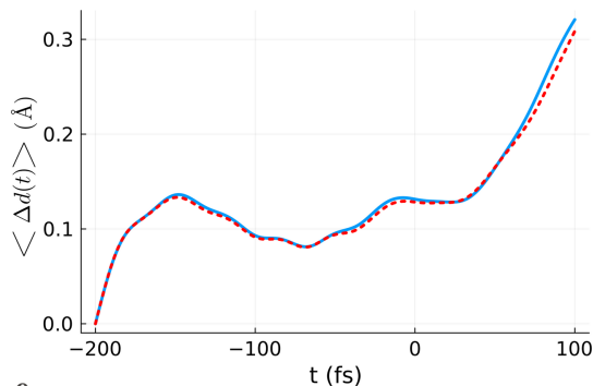
Figure 9 Comparison between the volume-integrated atomic displacement \langle \Delta d(t) \rangle_{\text{vol,real}} (blue line) and the atomic displacement calculated for the effective fluence averaged over 50 XTANT realizations (red line). The volume integration was performed for a silicon sample with 64 atoms in the simulation box, using the XTANT results for the doses marked in blue in Fig. 8, and assuming a pulse duration of 6 fs FWHM and photon energy of 50 eV. The same parameters were used for the effective dose simulation, except for the dose itself, set to D_{\text{eff}} = 4.20 \text{ eV atom}^{-1} .
