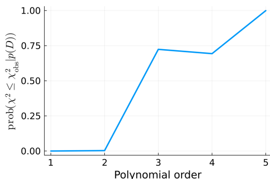
Figure 14 \text{prob}[\chi^2 \leq \chi_{\text{obs}}^2 | p(D)] from equation (13) calculated for the \chi^2 = \nu \chi_{\nu}^2 values present in Fig. 13.
