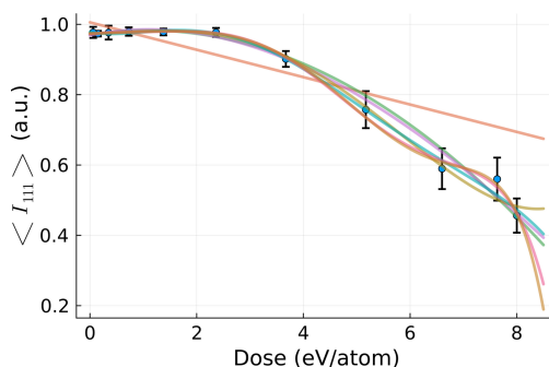
Figure 15 Polynomial fits of different orders performed for the data set [\sum_{i=1}^{10} D_i/10, \sum_{i=1}^{10} \langle F_{111}(D_i, t = t_{\text{final}}) \rangle_{\text{rel}}/10] , obtained from the simulations used to volume integrate the result in Fig. 5.
