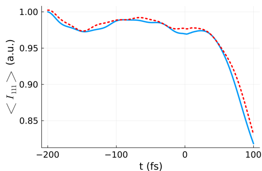
Figure 6 Comparison between the volume-integrated Bragg reflection intensity \langle I_{111}(t) \rangle_{\text{vol,real}} (blue line), and the Bragg reflection intensity obtained for the effective dose \langle I_{111}(t) \rangle_{\text{rel}} averaged over 50 XTANT realizations (red line). The volume integration was performed for a silicon sample with 64 atoms in the simulation box, using the XTANT results for the doses marked in blue in Fig. 1, and assuming a pulse duration of 6 fs FWHM and photon energy of 50 eV. The same parameters were used for the effective dose simulation, except for the dose itself, set to D_{\text{eff}} = 4.51 \text{ eV atom}^{-1} .
