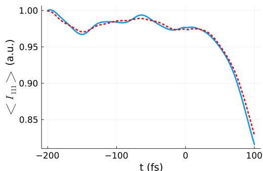
Figure 10 Comparison between the volume-integrated Bragg reflection intensity \langle I_{111}(t) \rangle_{\text{vol,real}} (blue line) and the Bragg reflection intensity calculated for an effective dose averaged over 50 XTANT realizations (red line). The volume integration was performed for a silicon sample with 64 atoms in the simulation box, using the XTANT results for the doses marked in blue in Fig. 8, and assuming a pulse duration of 6 fs FWHM and photon energy of 50 eV. The same parameters were used for the effective dose simulation, except for the dose itself, set to D_{\text{eff}} = 4.51 \text{ eV atom}^{-1} .
