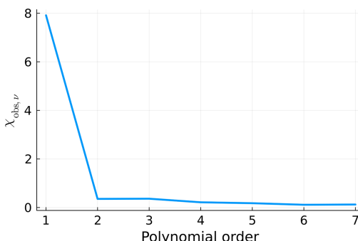
Figure 16 \chi_{\text{obs},\nu}^2 calculated for the fits displayed in Fig. 15.
