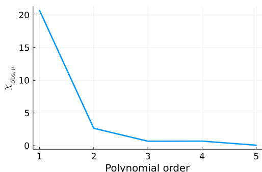
Figure 13 \chi_{\text{obs},\nu}^2 calculated for the fits displayed in Fig. 12.
