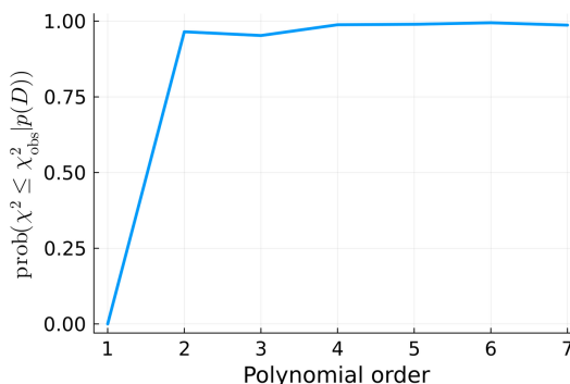
Figure 17 Parameter \text{prob}[\chi^2 \leq \chi_{\text{obs}}^2 | p(D)] from equation (13) calculated for the \chi^2 = \nu \chi_{\nu}^2 values as in Fig. 16.
