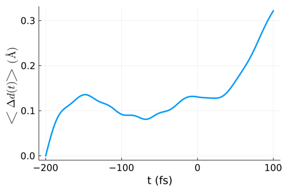
Figure 3 Volume-integrated and realization averaged atomic displacement \langle \Delta d(t) \rangle_{\text{vol,real}} . The integration was performed using the XTANT simulations performed for the doses marked in blue in Fig. 1. The calculation was performed for a silicon sample with 64 atoms in the simulation box, assuming a pulse duration of 6 fs FWHM and photon energy of 50 eV.
