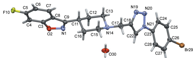
Figure 1 A view of the molecular structure of the title compound, with the atom labelling. Displacement ellipsoids are drawn at the 50% probability level.
