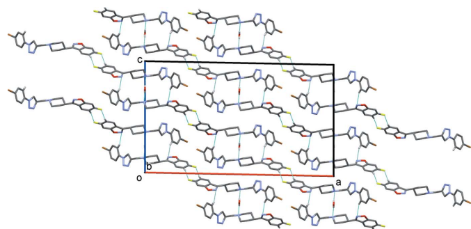
Figure 2 A view in projection along the b axis of the crystal packing of the title compound. Hydrogen bonds are shown as dashed lines (see Table 1), and H atoms not involved in hydrogen bonding have been omitted for clarity.
